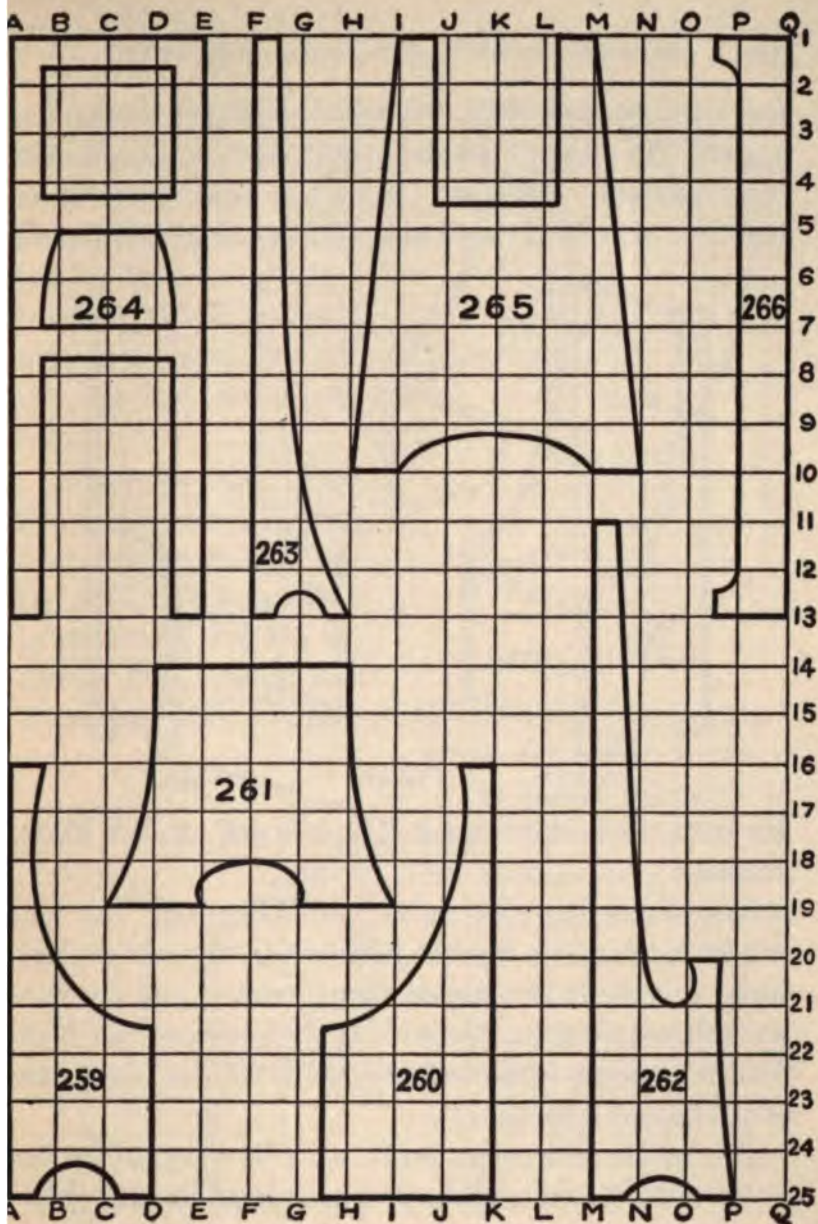
FIGS. 259-266. — Patterns for Furniture.
